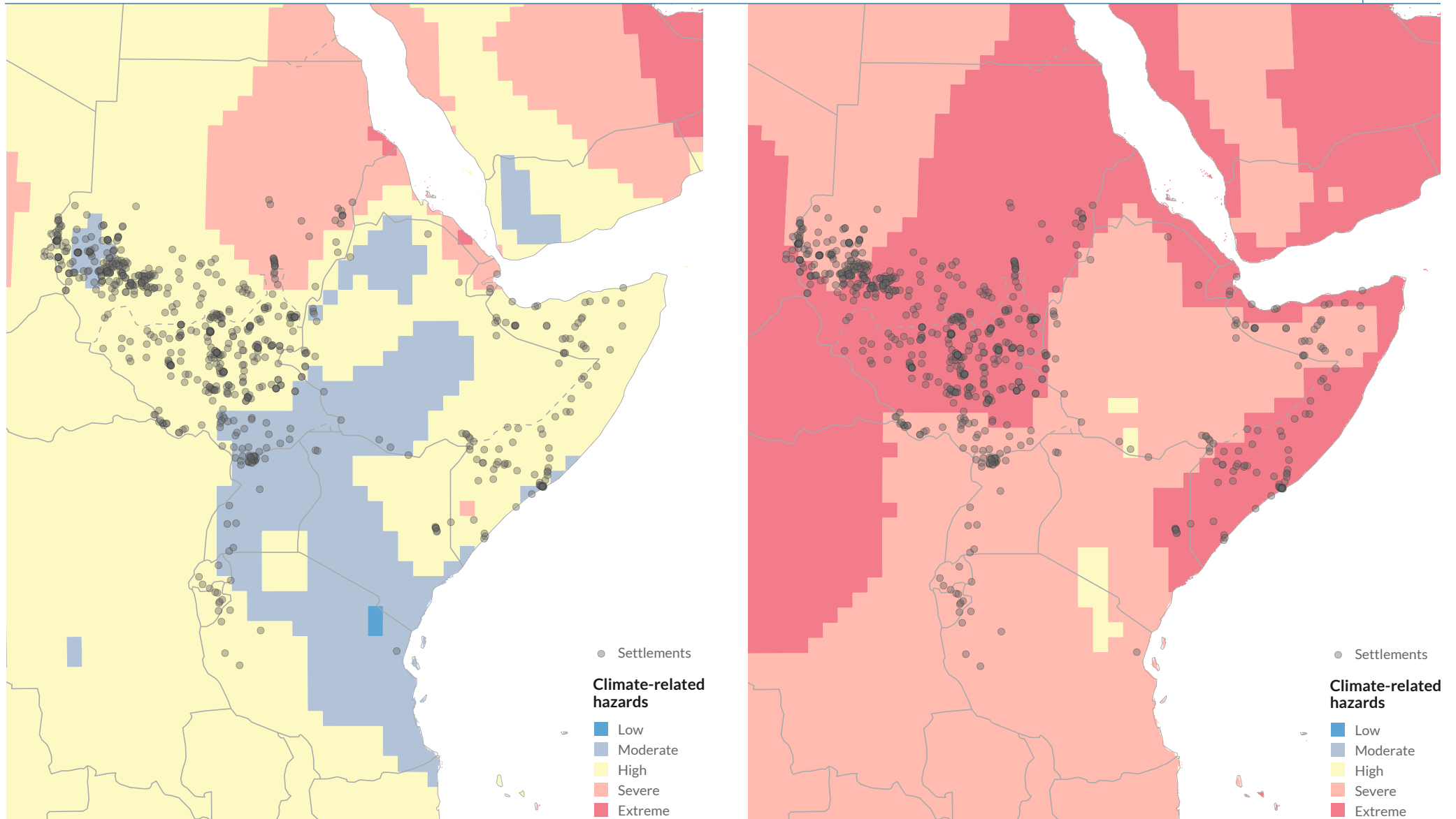
Figure 5: Exposure to compound climate-related hazards of formal and informal refugee and IDP settlements and camps in the East and Horn of Africa and the Great Lakes Region. The map on the left shows a baseline of current climate-related hazards, and the map on the right shows projections by 2040 (Craparo et al., forthcoming).
